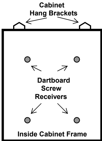
Cabinet Diagram
